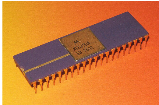
Motorola 6800, 1974
